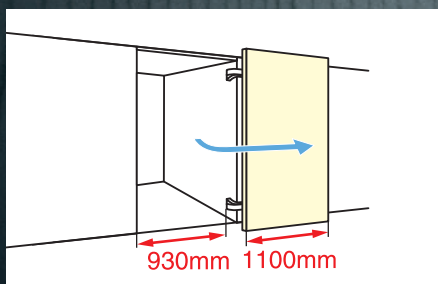
Minimal space required (max. door width 1,100 mm/effective opening width 930 mm). The door stays out of the way when opening and closing it.
