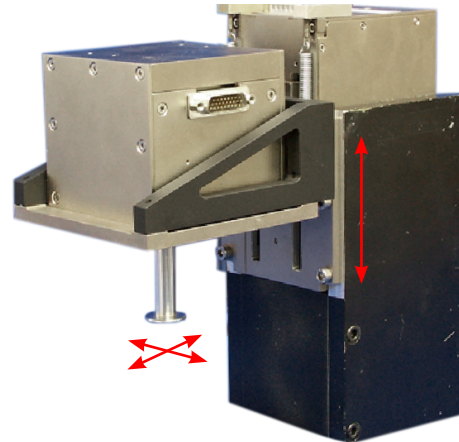
Multi-Axis LXY15 and LAS95 (3 Axes)
