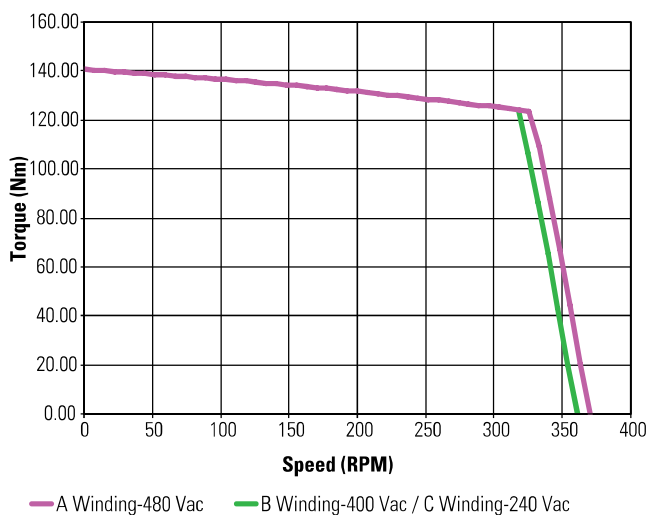
KBM(S)-79X03 ContinuousTorque
