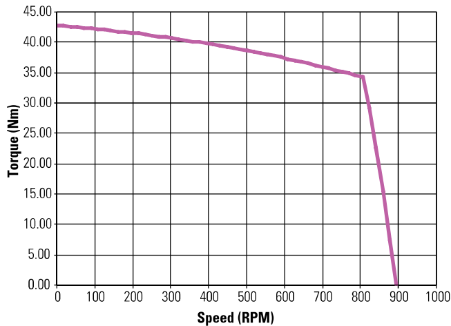
KBM(S)-79X01 ContinuousTorque
