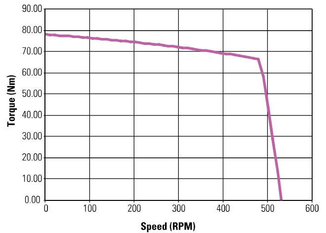
KBM(S)-79X02 ContinuousTorque
