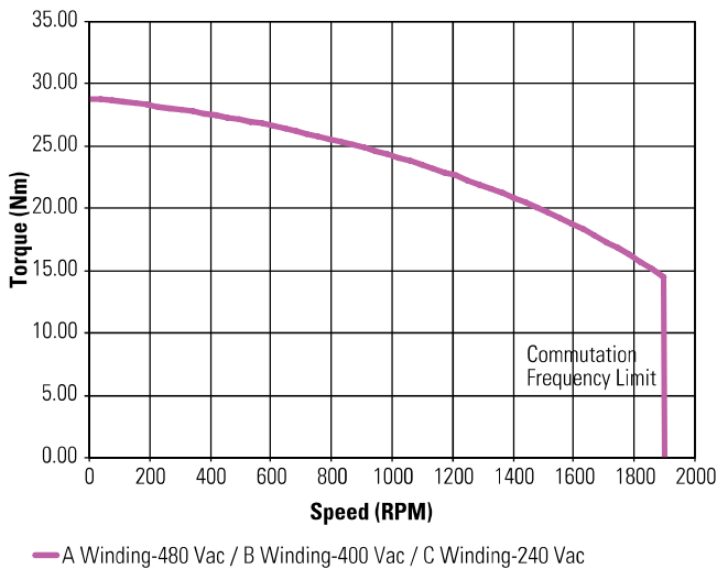
KBM(S)-60X00 Continuous Torque
