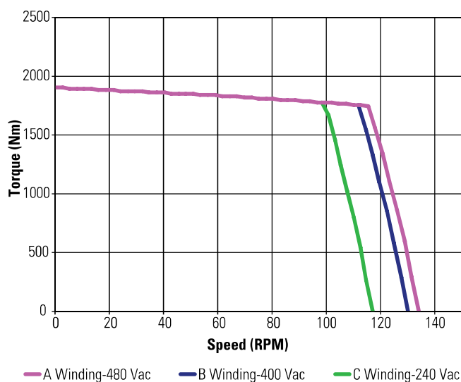
KBM(S)-260X01 ContinuousTorque
