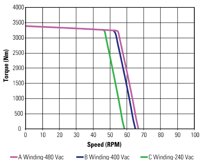
KBM(S)-260X03 ContinuousTorque
