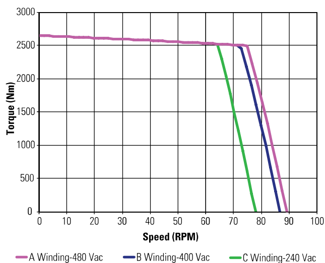
KBM(S)-260X02 ContinuousTorque
