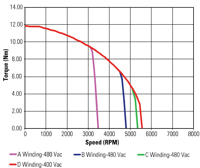
KBM(S)-25X03 ContinuousTorque
