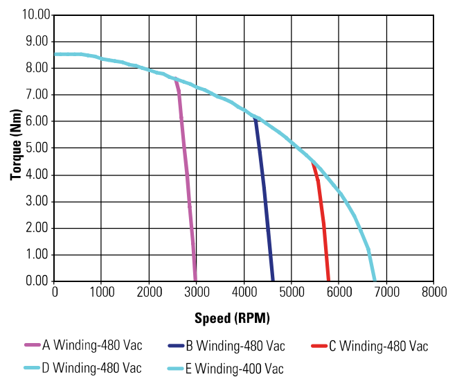
KBM(S)-25X02 ContinuousTorque
