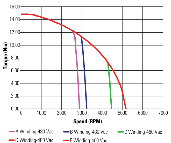
KBM(S)-25X04 ContinuousTorque
