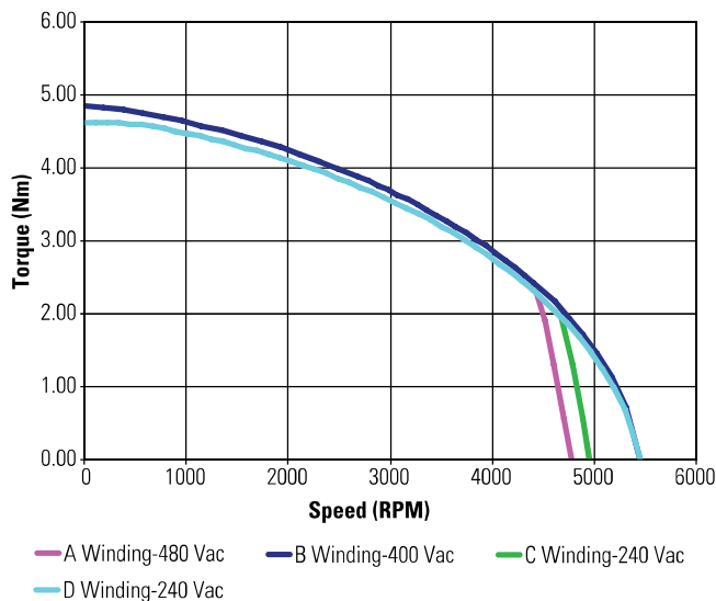
KBM(S)-25X01 ContinuousTorque
